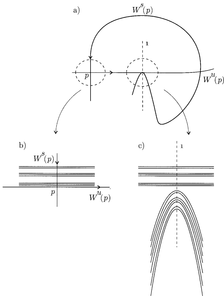
Figure 1.1 – Homoclinic tangency of stable and unstable manifolds emanating from a fixed point p
